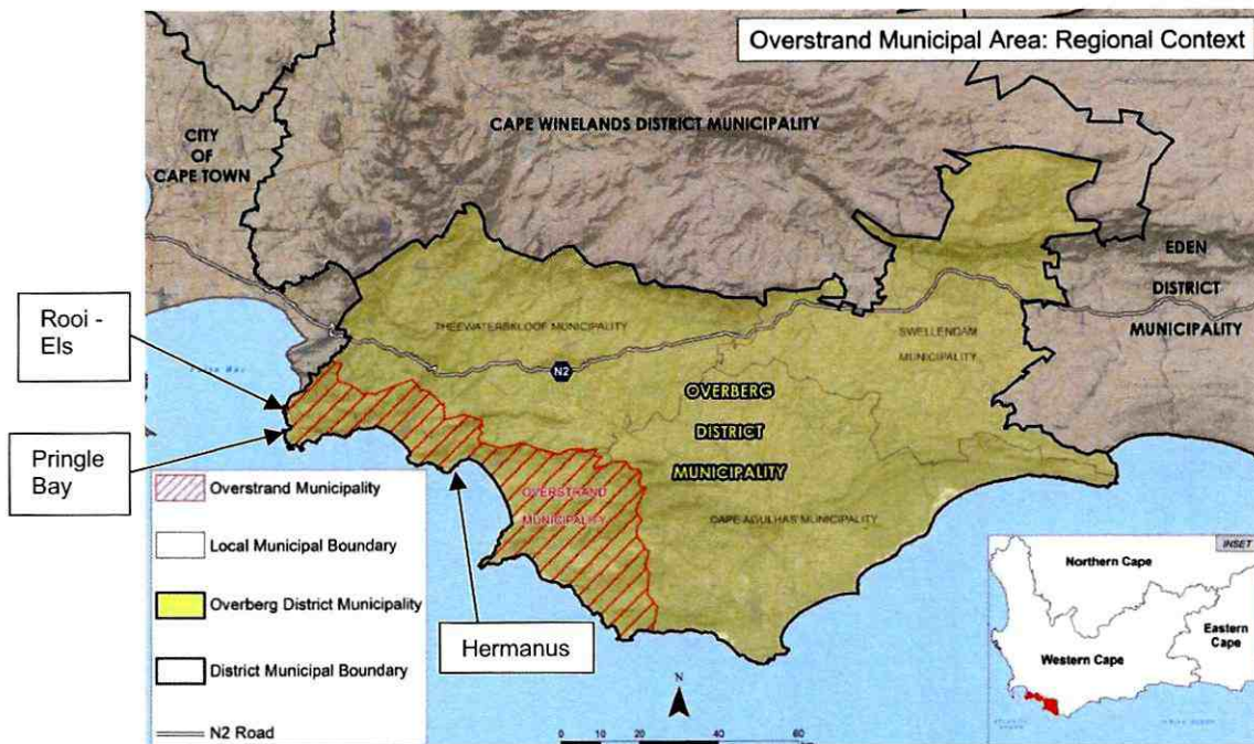
Figure 2: Regional Context
